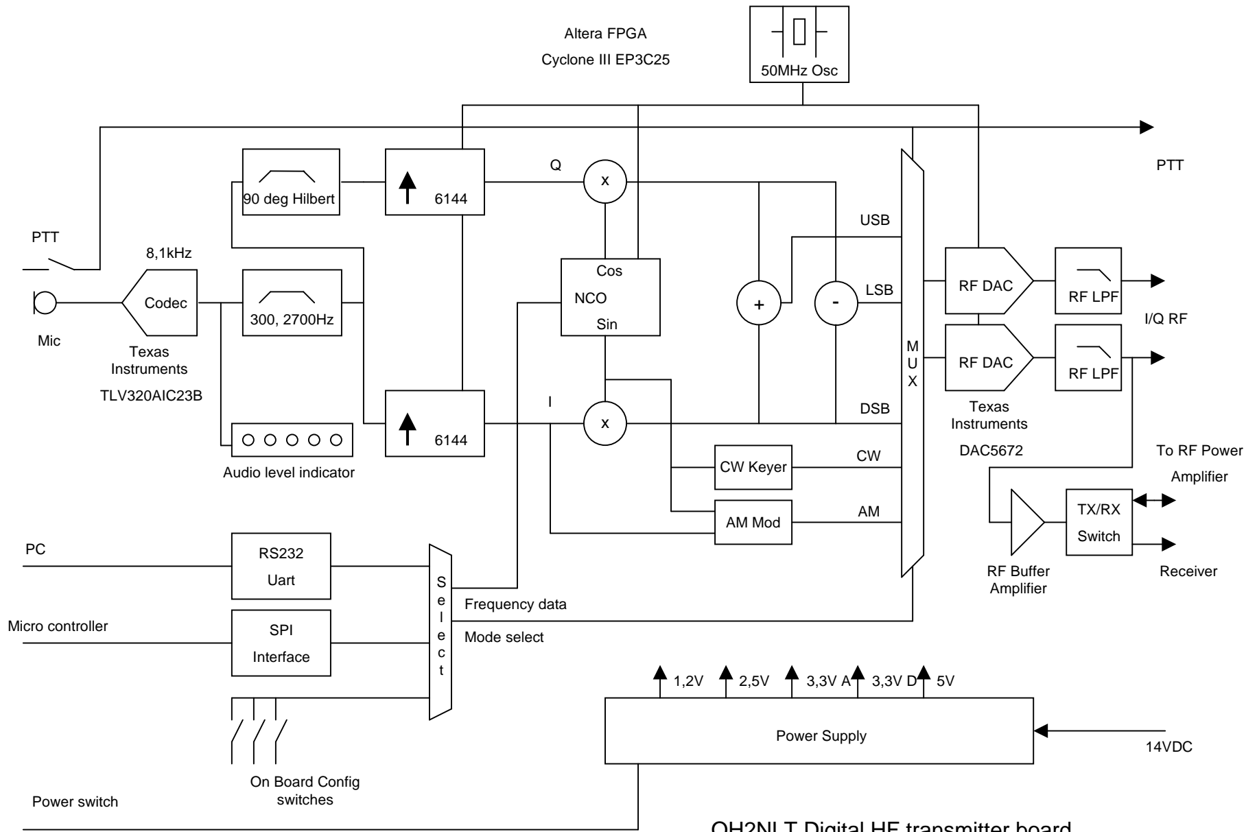
OH2NLT Digital HF transmitter board 19.12.2008
